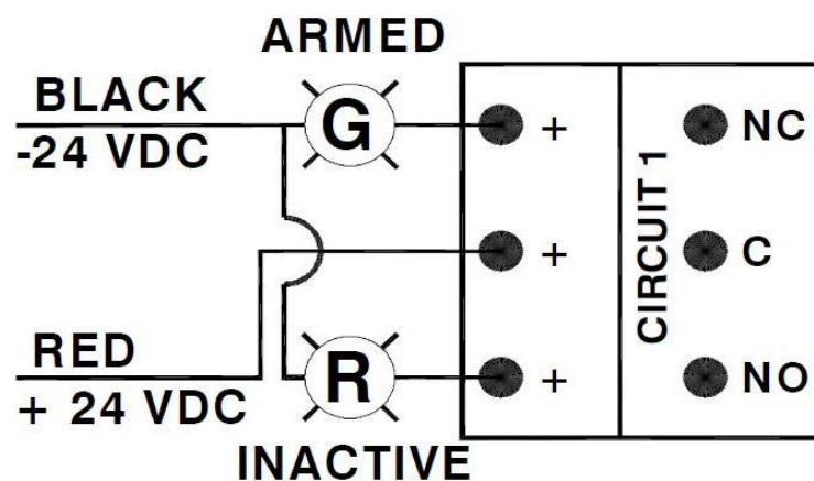
FIGURE 2. WIRING DIAGRAM
