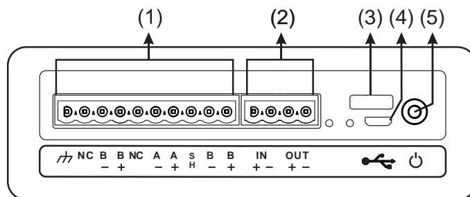
Figure 2: KI-HDT Terminal Connectors & Ports
